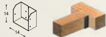
KS 14 Soflex Intermediate Beam Bracket
