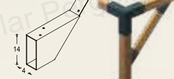
KP 49 45 flex Buttress Bracket
