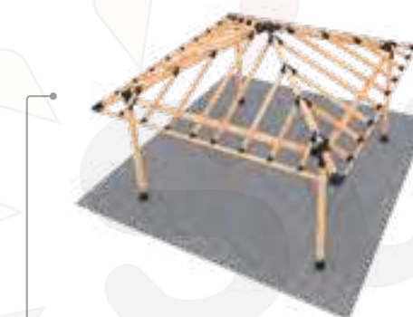
Roof 20 with Roof and Eaves 9x9 - 14x14 PAGE 28
