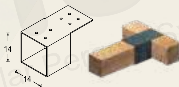
KC 14 Colflex Intermediate Beam Bracket
