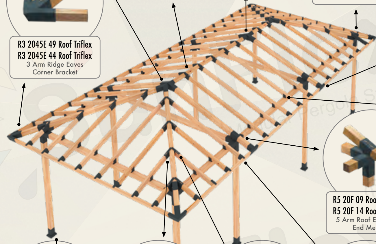
R4 2045F 09 Roof Tetraflex R4 2045F 14 Roof Tetraflex 4 Arm Roof Open Ended Corner
