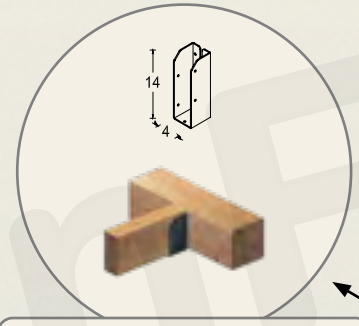
KS 44 Soflex Intermediate Beam Bracket
