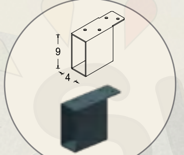
KC 49 Colflex Intermediate Beam Bracket
