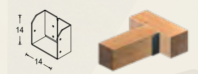
KS 14 Soflex Intermediate Beam Bracket
