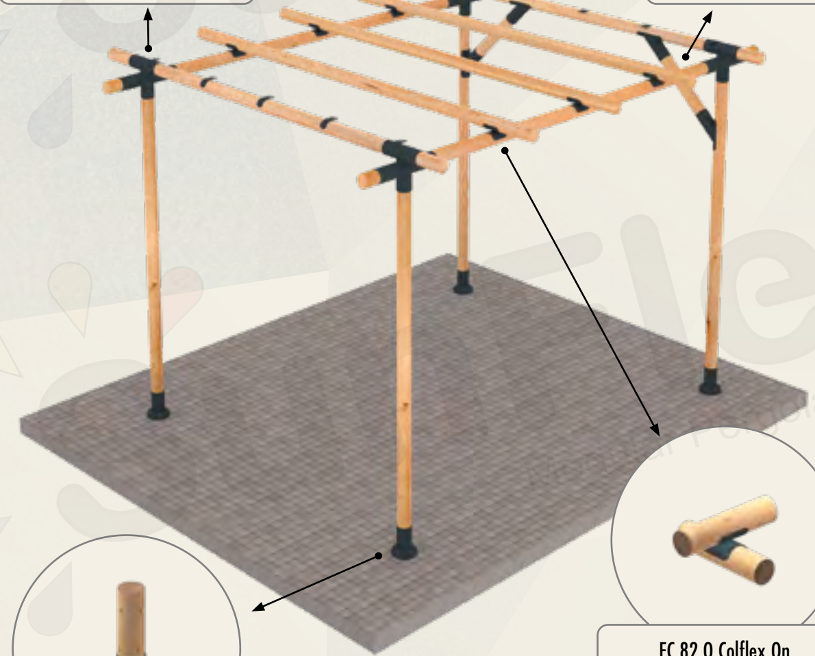
EC 82 0 Colflex On 3 Arm Edge Middle Bracket
