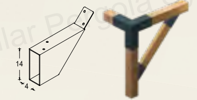
KP 49 45 flex Buttress Bracket
